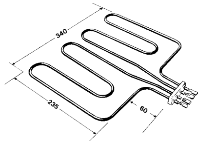
1929 2 x 1000W Grill Elements Replaces - Email 90729
