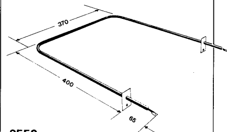
2559 2200W Oven Element Replaces - Email VF040000
