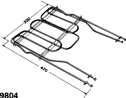
9804 3100/750W Grill/Bake Element Replaces - F&P 461368
