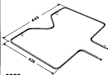
9983 2250W Bake Element Replaces - F&P 572015
