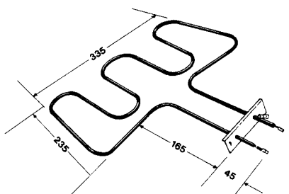
2558 2000W Grill Element Replaces - Email VF080000
