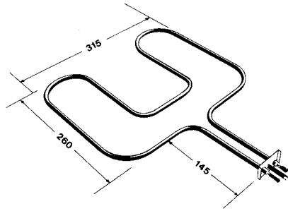
1272 2400W Grill Element
