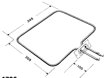
1796 2200W Oven Element Replaces - Email 42047
