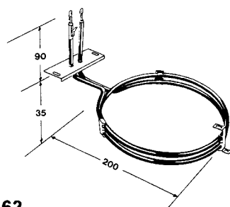
2462 2200W Fan Forced Oven Element Replaces - Email 823271
