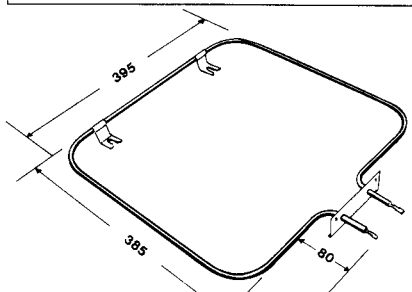
2545 2200W Oven Element Replaces - Email 90155
