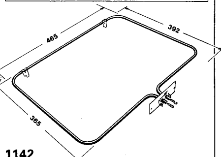
1142 3000W Oven Element Replaces - Chef 03743
