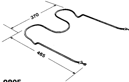
9805 2250W Oven Element (bottom) Replaces - F&P 461095
