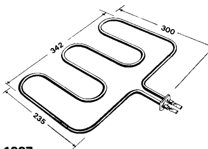
1887 2000W Oven Element Replaces - Email 90680
