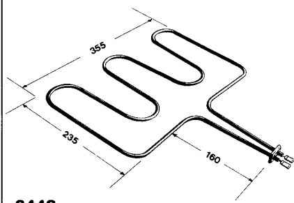
2448 2000W Grill Element Replaces - Email 91074
